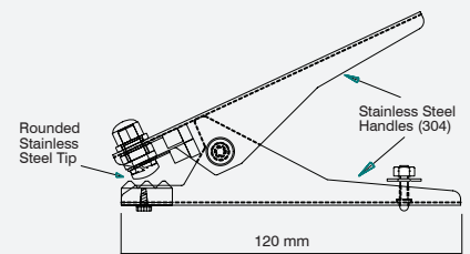
FIBC Monitoring Clamp
